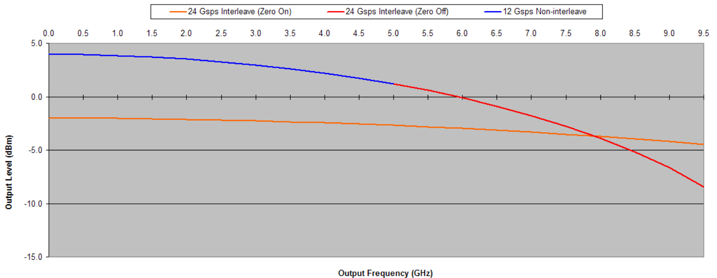
AWG7122C Frequency Response, Includes \sin x/x Rolloff
