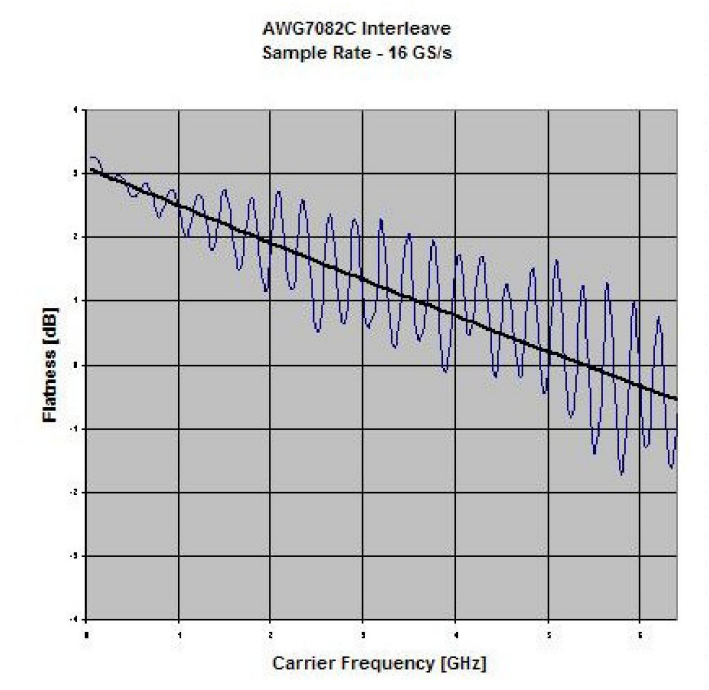
AWG7082C Interleave Flatness (typical).
