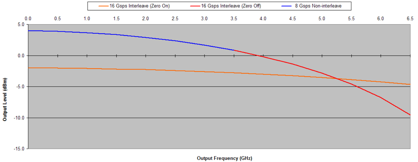
AWG7082C Frequency Response, Includes \sin x/x Rolloff
