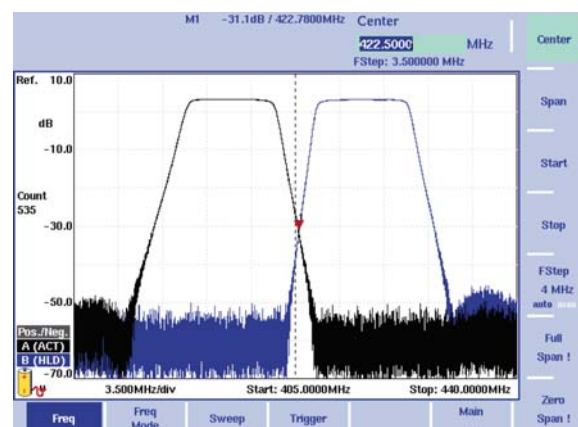
Isolation between receive and transmit stages
