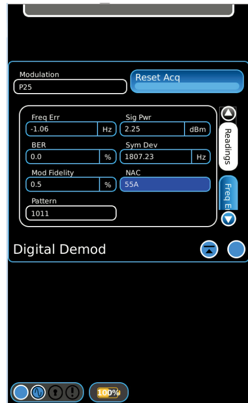
The 3550 Digital Analysis Panel
