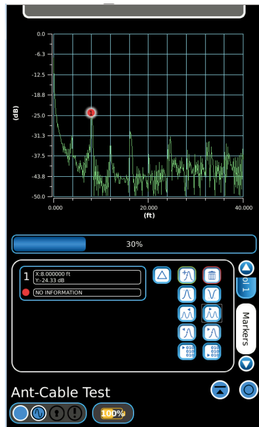
The 3550 Distance To Fault Analysis
